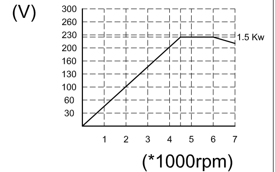
Power-diagram
