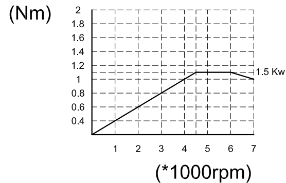
Torque-diagram
